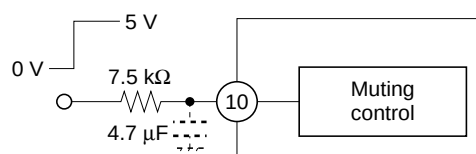
Figure 2 How to use Muting Circuit
