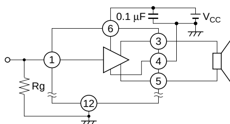
Figure 1 Notes on Application Board's Pattern Design
